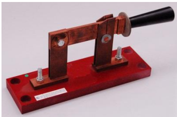
Knife switch connects to the positive side of the welder for cutting current during change of consumables.
